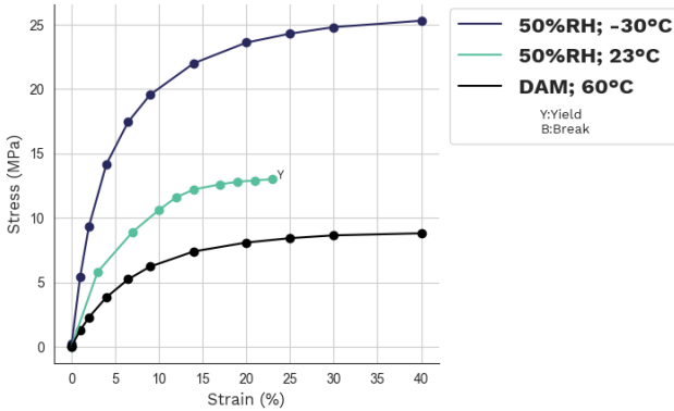
Stress-strain Pebax® 5533 SP 01
